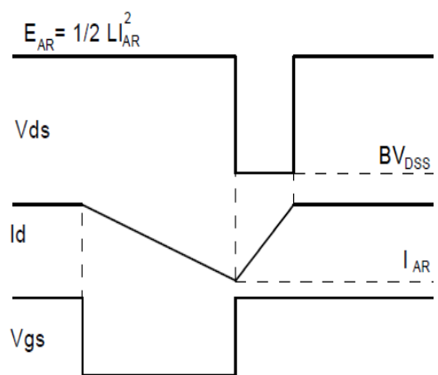
Fig.3-2 Avalanche waveform
