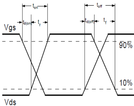
Fig.1-2 Switching Waveform
