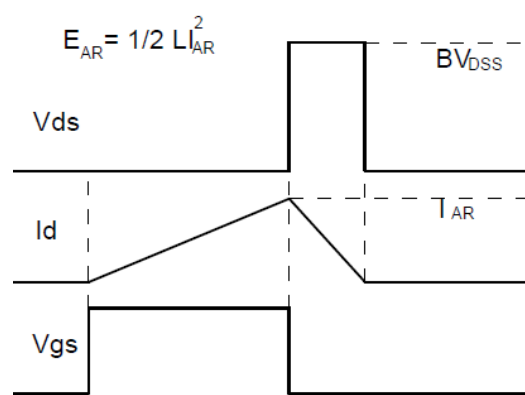
Fig.3-2 Avalanche waveform
